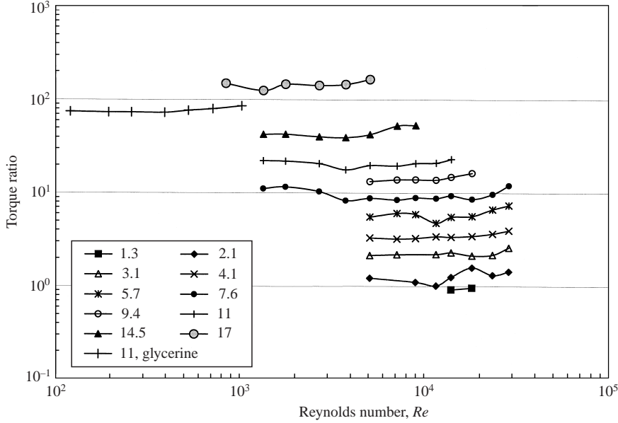
FIGURE 7. The ratio of Bagnold's measured torque using water, M_{Bag} , to torque calculated for laminar boundary layer flow over a spinning disk, M_{bl} for different values of \lambda . The data for the glycerin mixture are for the ratio of M_{Bag} to M_{shear} .
